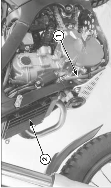
(1) OVERFLOW HOSE (2) RADIATOR
