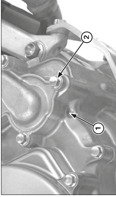
(1) INSPECTION HOLE (2) COOLANT DRAIN BOLT/SEALING WASHER
